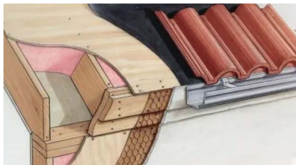
CLAY TILE ROOF ASSEMBLY
